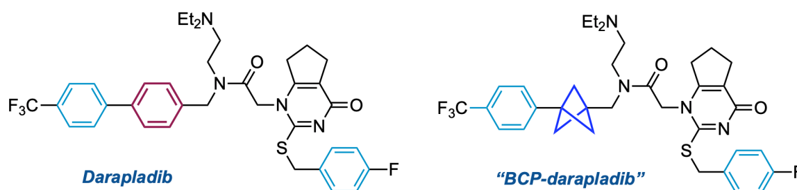
Figure 1: Molecular structures of darapladib (left) and BCP-darapladib (right) with benzene rings shown in light blue and key benzene and BCP rings shown in purple and dark blue respectively.
