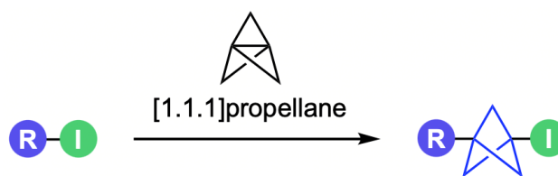
Figure 2: Insertion of [1.1.1]propellane into an organic halide.
