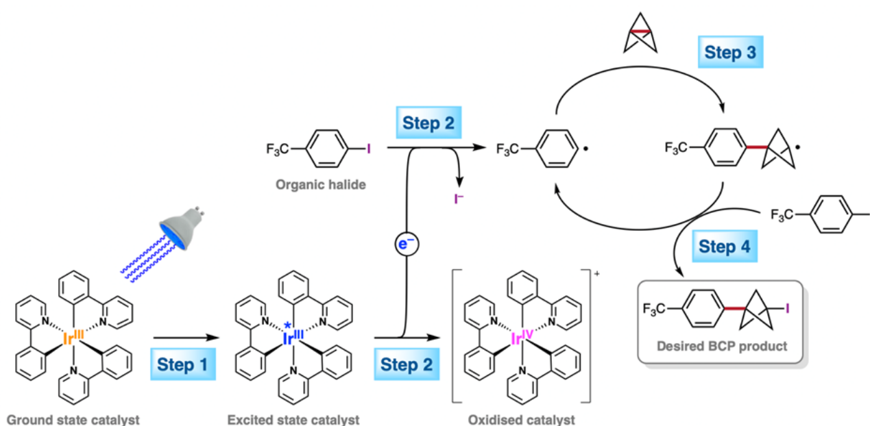
Figure 3: Reaction mechanism of the radical process.
